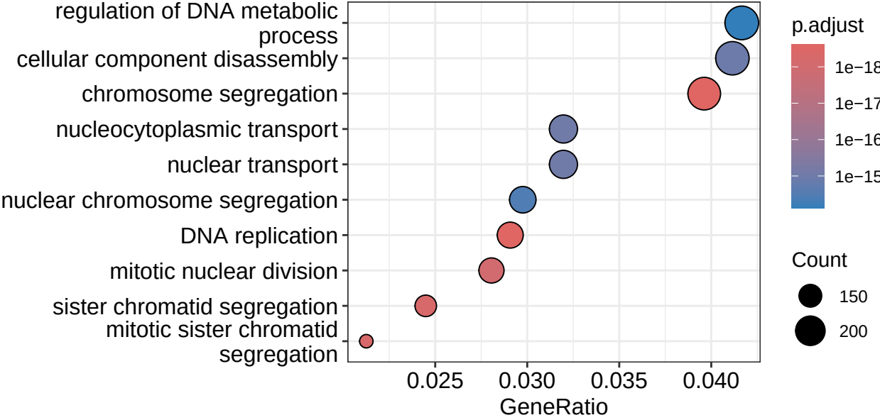
GO Enrichment
